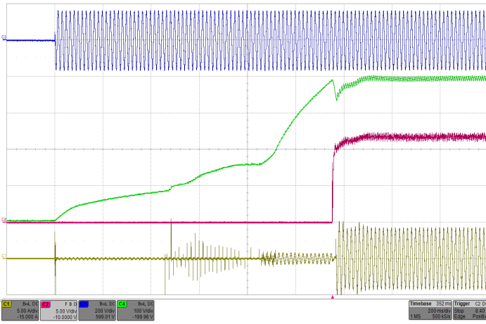
Figure 13: Typical startup waveform with 200µF hold-up capacitor (115Vrms, 60Hz) Top: Vin (200V/div), Top Middle: Hold-up capacitor voltage (100V/div), Bottom Middle: Vout (5V/div), Bottom: Iin (5A/div), Timebase: (200ms/div).
