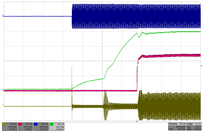
Figure 14: Typical startup waveform with 200µF hold-up capacitor (115Vrms, 400Hz) Top: Vin (200V/div), Top Middle: Hold-up capacitor voltage (100V/div), Bottom Middle: Vout (5V/div), Bottom: Iin (5A/div), Timebase: (200ms/div).
