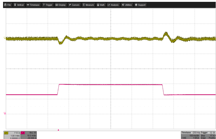
Figure 12: Regulated model output voltage response to step-change in load current with 200µF hold-up capacitor (50%-75%-50% of Iout(max), 115Vrms, 400Hz) Top: Vout (1V/div), Bottom: Iout (10A/div), Timebase: (100ms/div).
