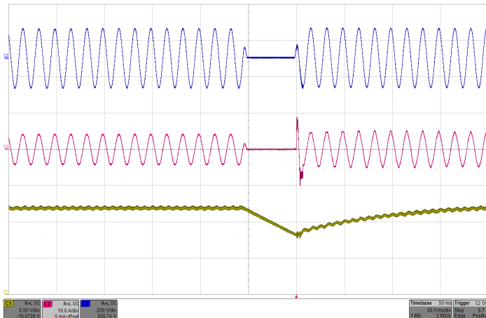
Figure 9: Line drop out with 400µF hold-up capacitor at full load current (115Vrms, 60Hz) Top: Vin (200V/div), Mid: Iin (10A/div), Bottom: Vout (5V/div), Timebase: (50ms/div).
