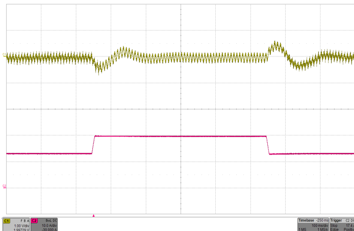
Figure 11: Regulated model output voltage response to step-change in load current with 200µF hold-up capacitor (50%-75%-50% of Iout(max), 115Vrms, 60Hz) Top: Vout (1V/div), Bottom: Iout (10A/div), Timebase: (100ms/div).
