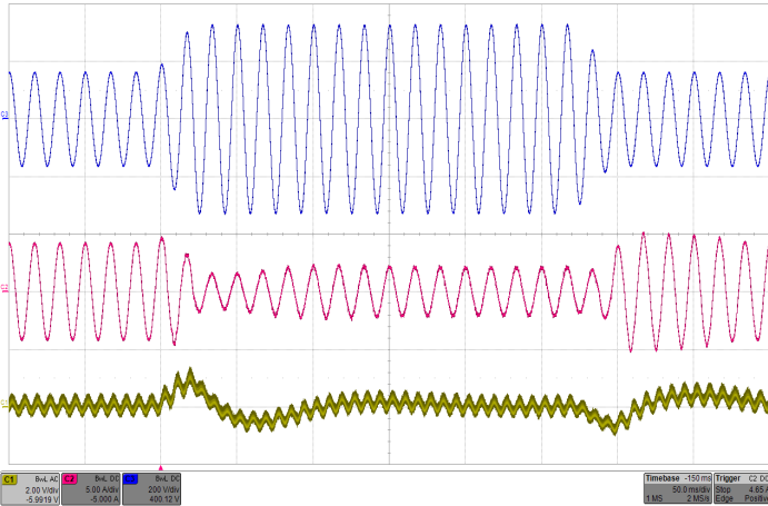
Figure 15: Input voltage transient response with 200µF hold-up capacitor at full load current (115Vrms-230Vrms-115Vrms, 60Hz), Top: Vin (200V/div), Mid: Iin (5A/div), Bottom: Vout (2V/div), Timebase: (50ms/div).
