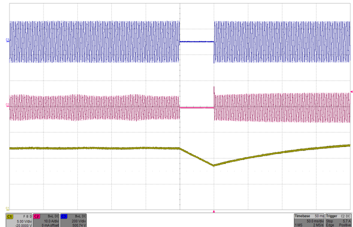
Figure 10: Line drop out with 400µF hold-up capacitor at full load current (115Vrms, 400Hz) Top: Vin (200V/div), Mid: Iin (10A/div), Bottom: Vout (5V/div), Timebase: (50ms/div).
